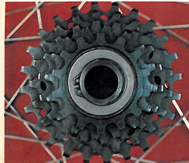
CLUSTER: Carries a full roller bearing assembly and is designed for silent running. Ratio—14-24. (Pat. Pend.)
